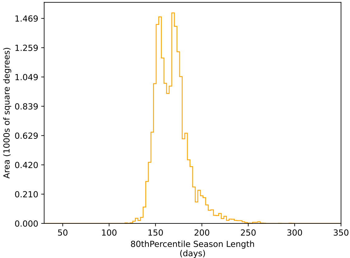
too_elab_r8_d3_gz_v3.4_10yrs WFD r band: 80thPercentile Season Length
