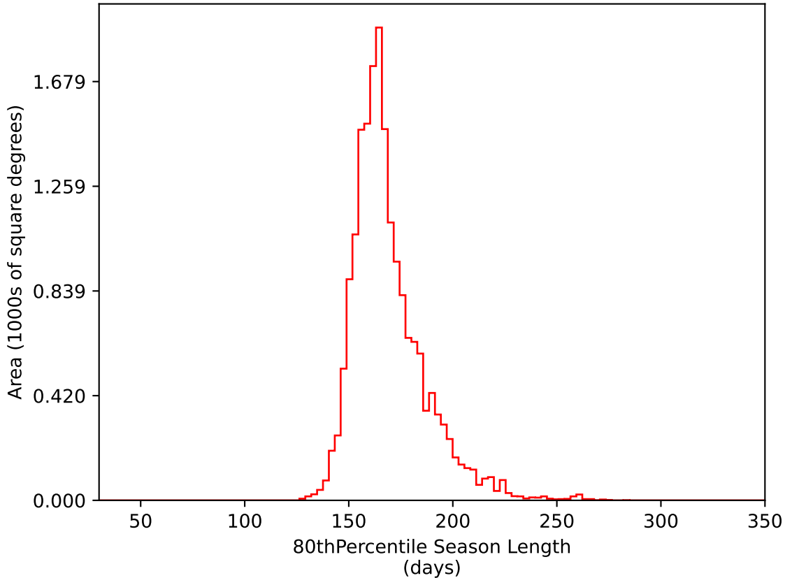
too_elab_r8_d3_gz_v3.4_10yrs WFD i band: 80thPercentile Season Length
