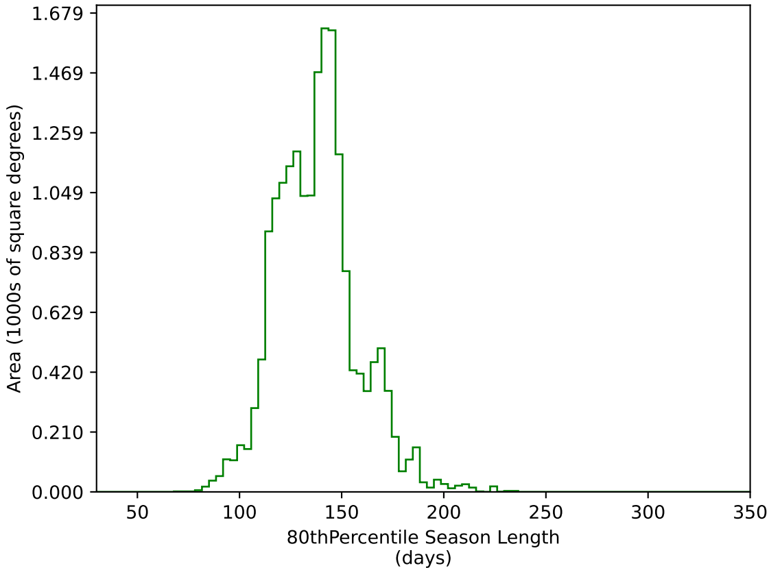
too_elab_r8_d3_gz_v3.4_10yrs WFD g band: 80thPercentile Season Length
