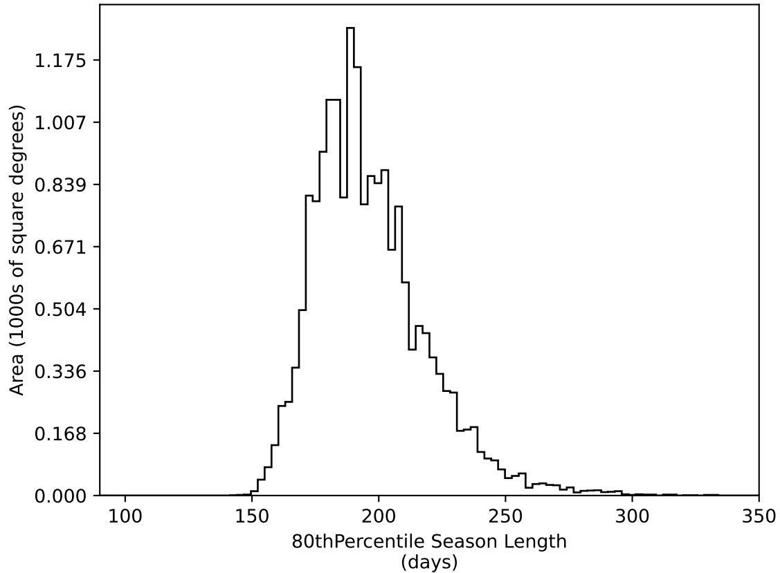
too_elab_r8_d3_gz_v3.4_10yrs WFD all bands: 80thPercentile Season Length
