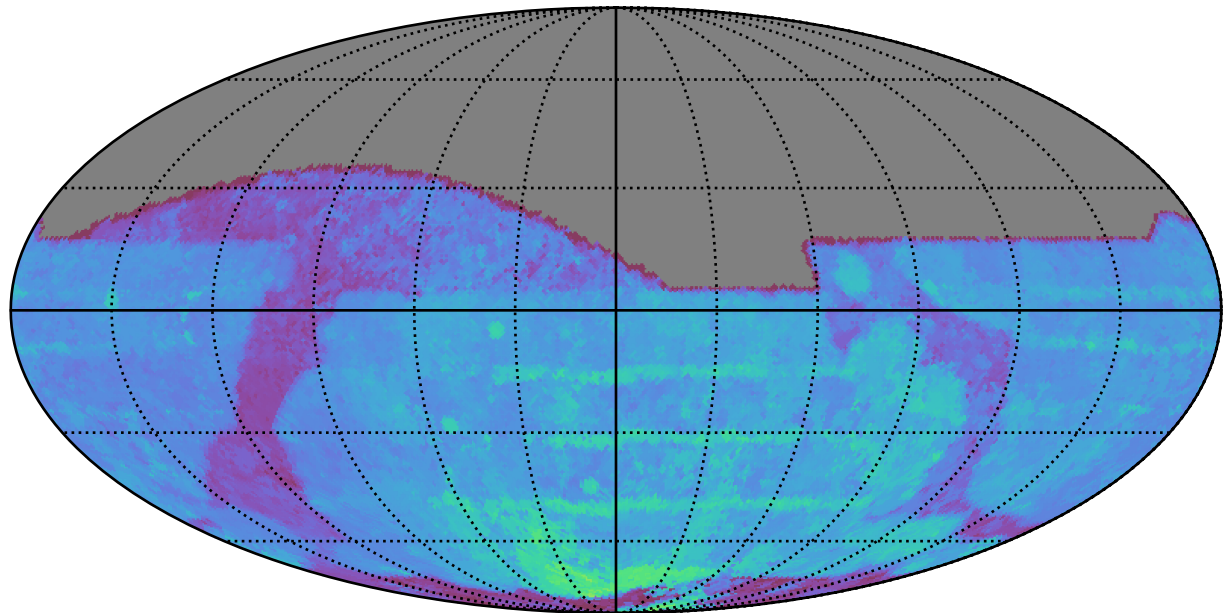
too_elab_r8_d3_gz_v3.4_10yrs All sky z band: 80thPercentile Season Length
