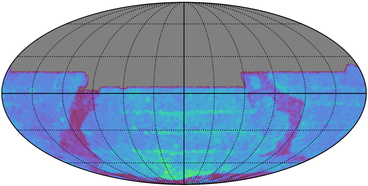
too_elab_r8_d3_gz_v3.4_10yrs All sky y band: 80thPercentile Season Length
