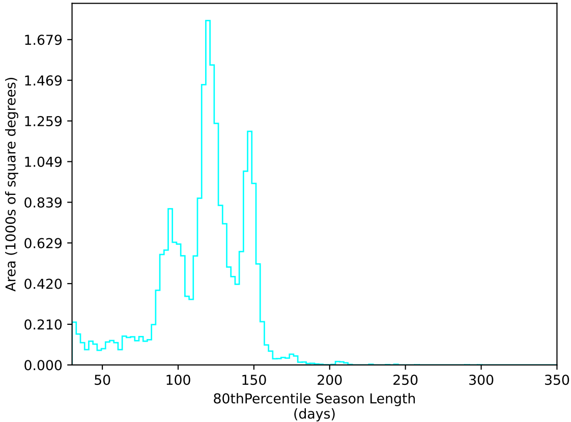
too_elab_r8_d3_gz_v3.4_10yrs All sky u band: 80thPercentile Season Length
