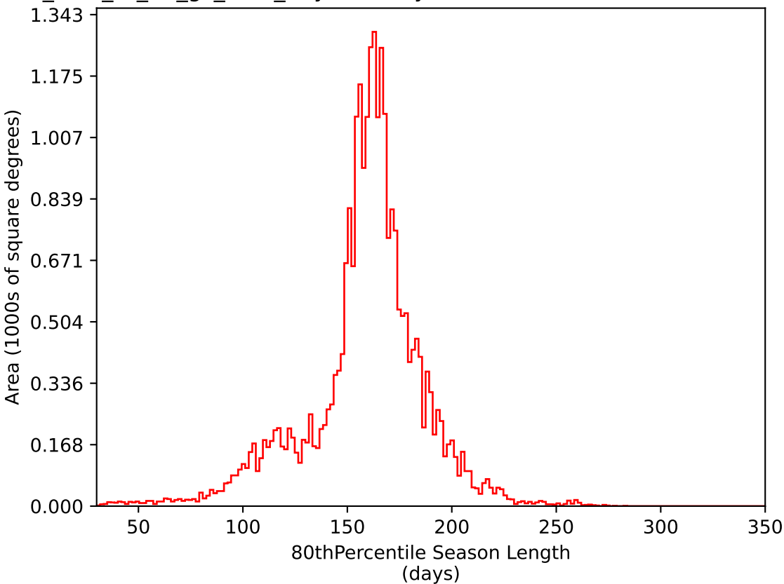
too_elab_r8_d3_gz_v3.4_10yrs All sky i band: 80thPercentile Season Length
