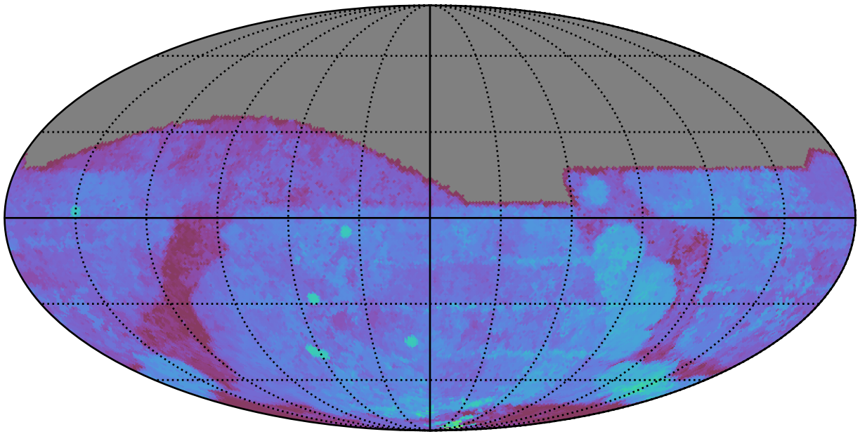
too_elab_r8_d3_gz_v3.4_10yrs All sky g band: 80thPercentile Season Length
