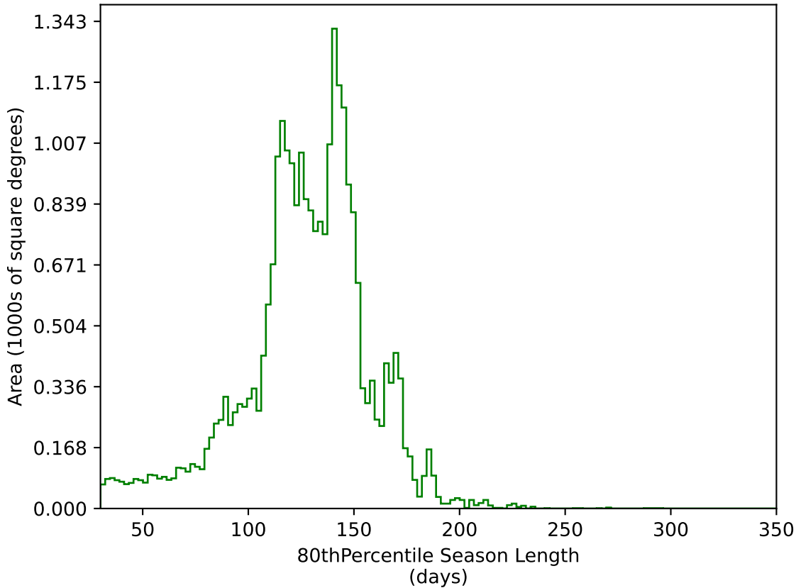
too_elab_r8_d3_gz_v3.4_10yrs All sky g band: 80thPercentile Season Length
