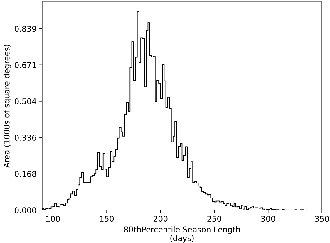
too_elab_r8_d3_gz_v3.4_10yrs All sky all bands: 80thPercentile Season Length
