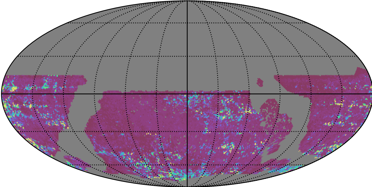
too_elab_r8_d3_gz_v3.4_10yrs WFD z band: 75th Percentile Intranight Timespan
