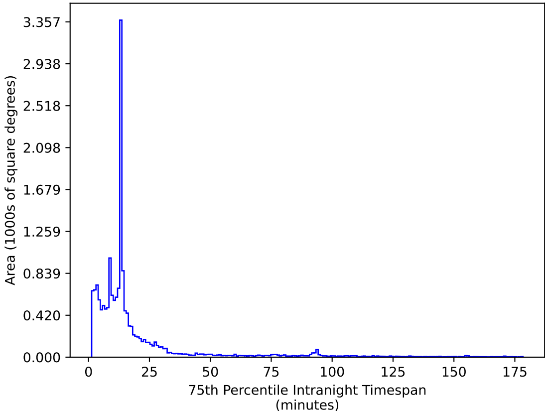
too_elab_r8_d3_gz_v3.4_10yrs WFD z band: 75th Percentile Intranight Timespan
