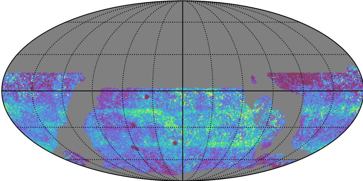
too_elab_r8_d3_gz_v3.4_10yrs WFD y band: 75th Percentile Intranight Timespan
