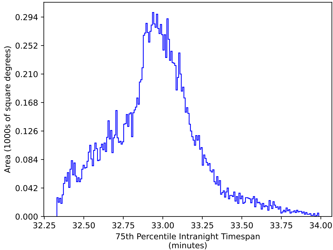
too_elab_r8_d3_gz_v3.4_10yrs WFD y band: 75th Percentile Intranight Timespan
