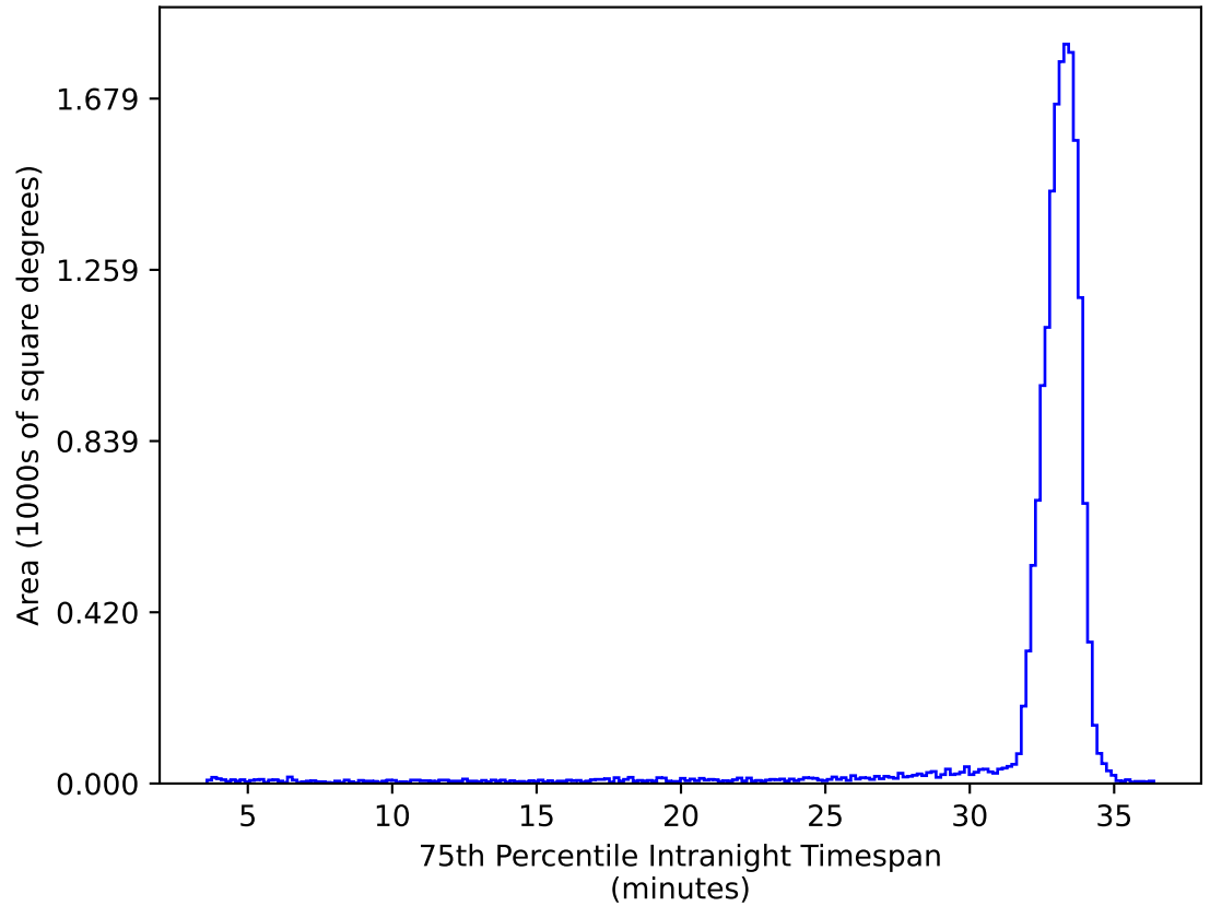
too_elab_r8_d3_gz_v3.4_10yrs WFD ug bands: 75th Percentile Intranight Timespan
