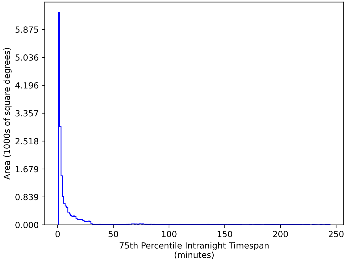
too_elab_r8_d3_gz_v3.4_10yrs WFD u band: 75th Percentile Intranight Timespan
