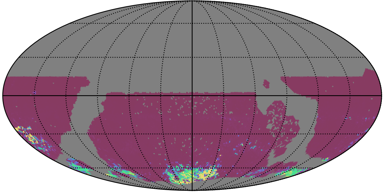
too_elab_r8_d3_gz_v3.4_10yrs WFD ri bands: 75th Percentile Intranight Timespan
