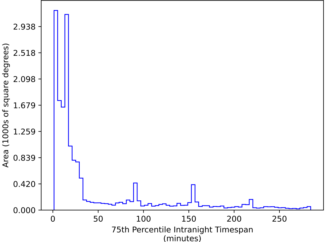
too_elab_r8_d3_gz_v3.4_10yrs WFD r band: 75th Percentile Intranight Timespan
