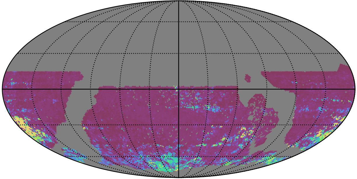
too_elab_r8_d3_gz_v3.4_10yrs WFD i band: 75th Percentile Intranight Timespan
