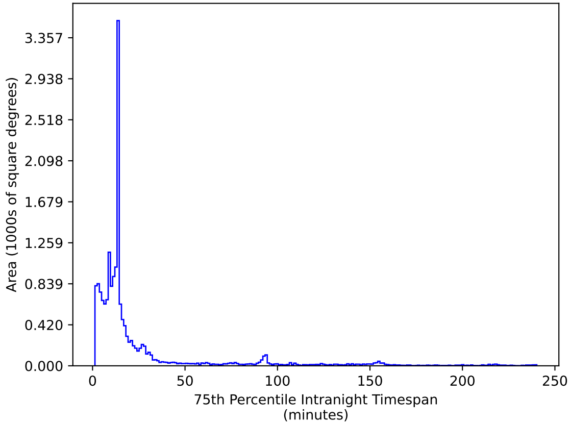
too_elab_r8_d3_gz_v3.4_10yrs WFD i band: 75th Percentile Intranight Timespan
