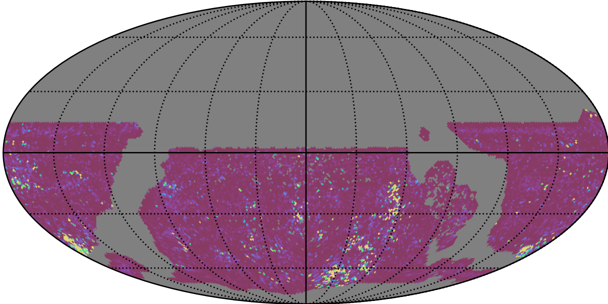
too_elab_r8_d3_gz_v3.4_10yrs WFD g band: 75th Percentile Intranight Timespan
