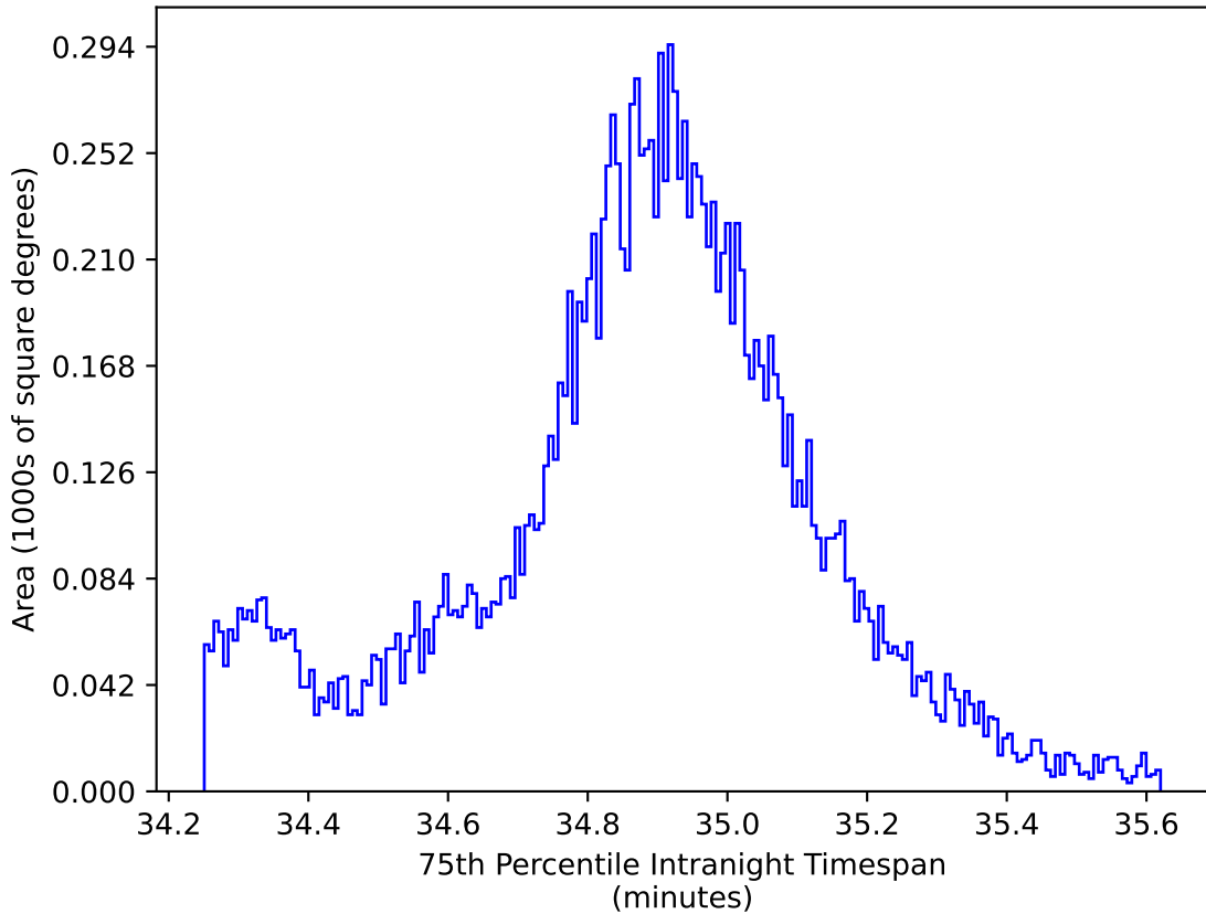
too_elab_r8_d3_gz_v3.4_10yrs WFD: 75th Percentile Intranight Timespan
