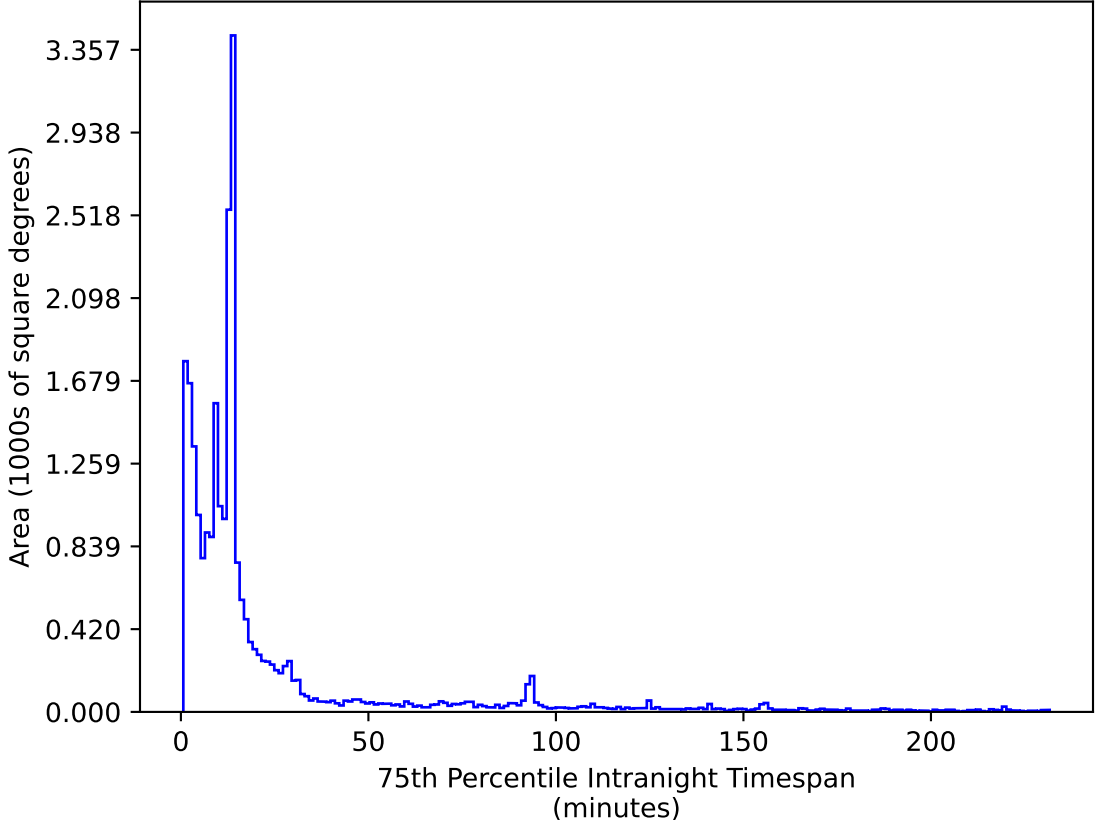
too_elab_r8_d3_gz_v3.4_10yrs All sky z band: 75th Percentile Intranight Timespan
