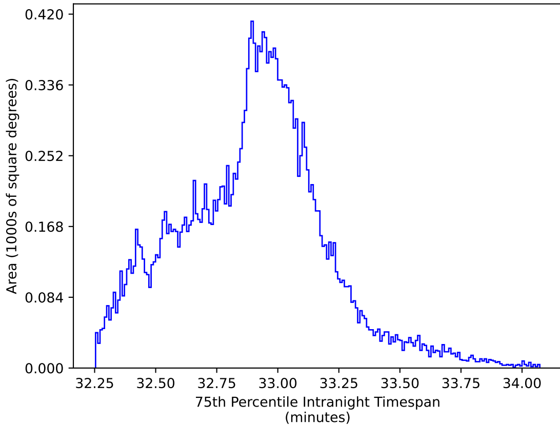
too_elab_r8_d3_gz_v3.4_10yrs All sky y band: 75th Percentile Intranight Timespan
