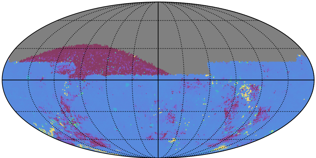
too_elab_r8_d3_gz_v3.4_10yrs All sky ug bands: 75th Percentile Intranight Timespan
