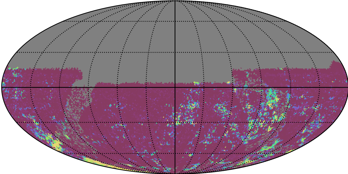
too_elab_r8_d3_gz_v3.4_10yrs All sky u band: 75th Percentile Intranight Timespan
