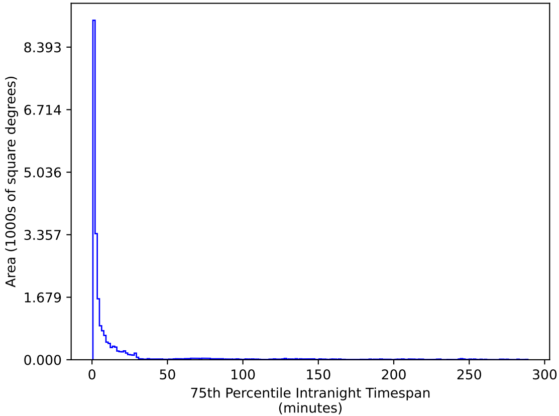
too_elab_r8_d3_gz_v3.4_10yrs All sky u band: 75th Percentile Intranight Timespan
