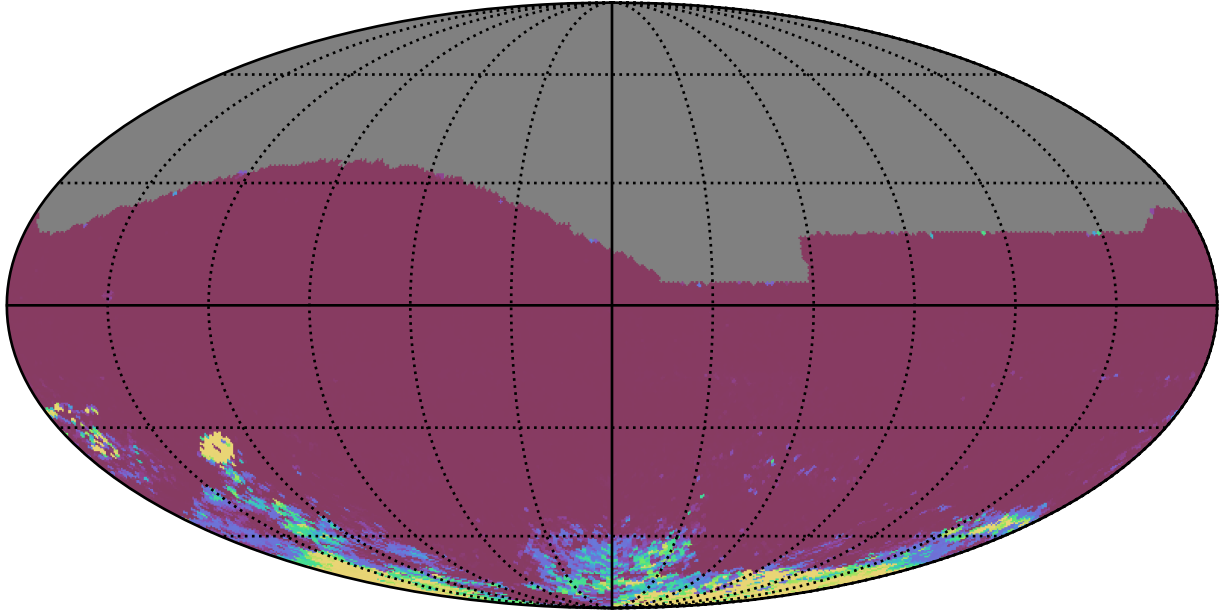
too_elab_r8_d3_gz_v3.4_10yrs All sky ri bands: 75th Percentile Intranight Timespan
