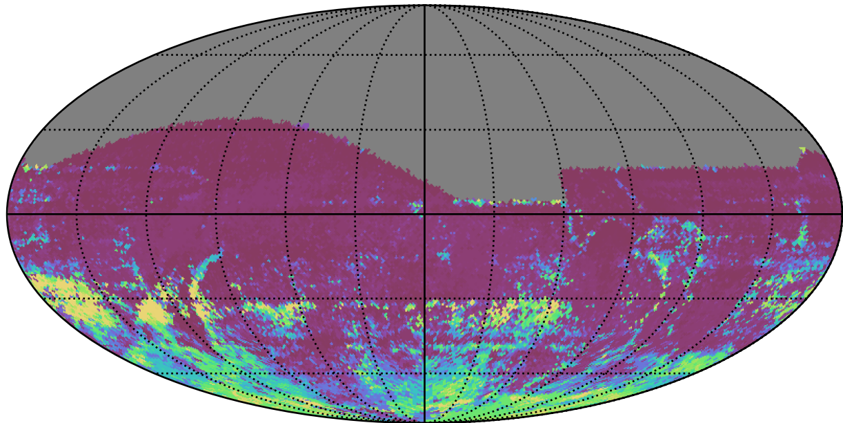
too_elab_r8_d3_gz_v3.4_10yrs All sky r band: 75th Percentile Intranight Timespan
