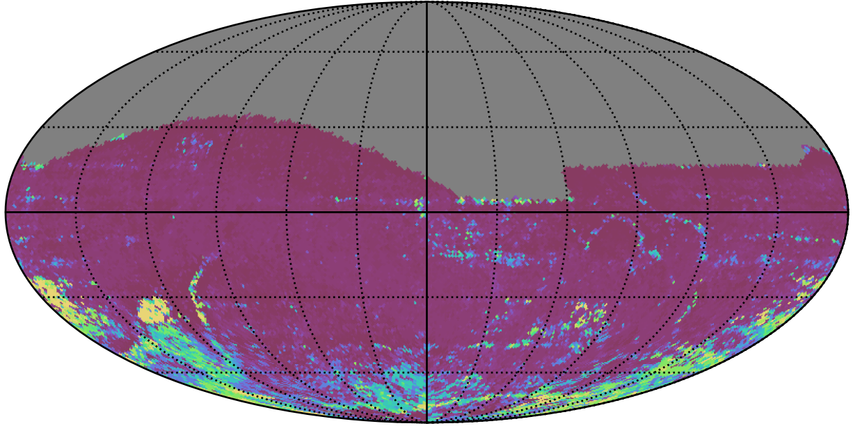
too_elab_r8_d3_gz_v3.4_10yrs All sky i band: 75th Percentile Intranight Timespan
