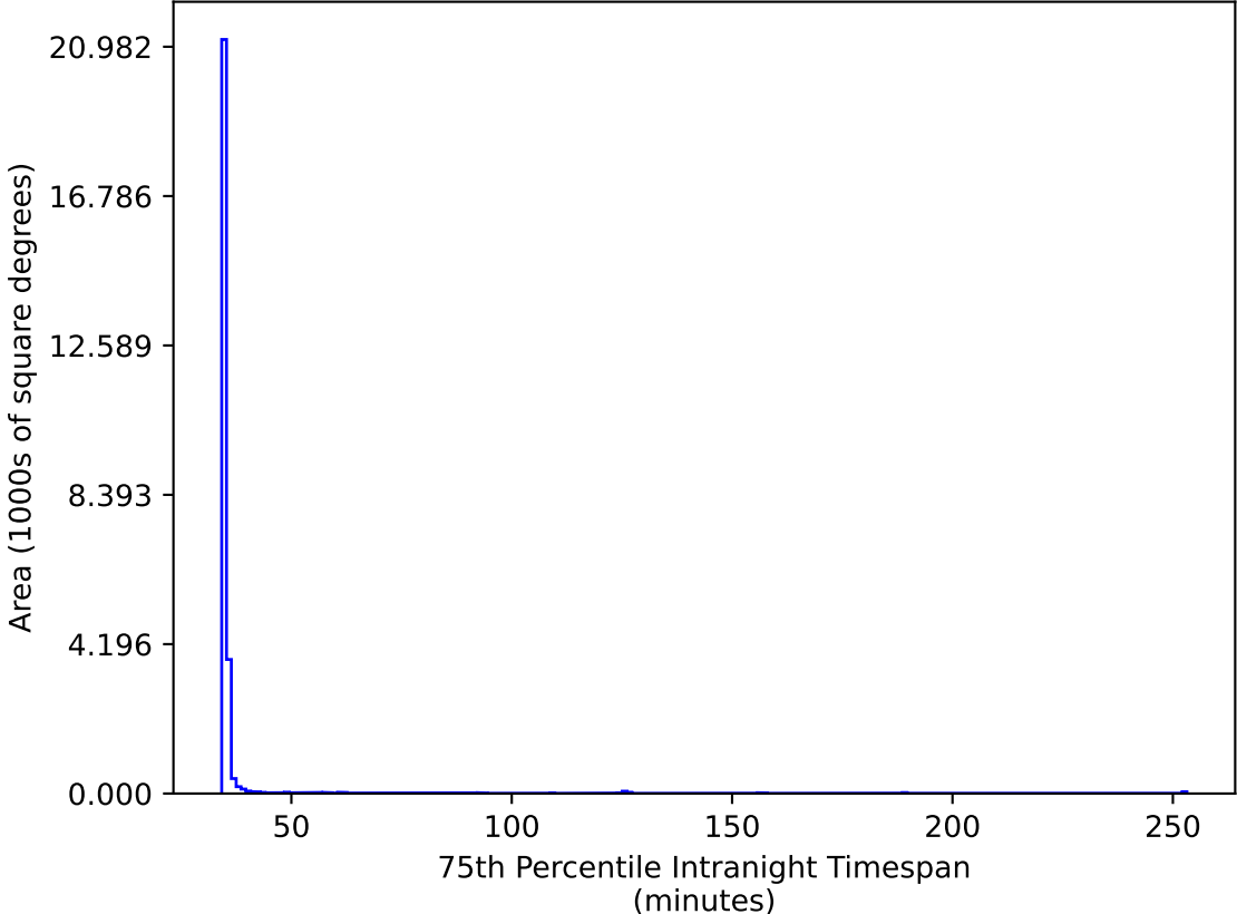
too_elab_r8_d3_gz_v3.4_10yrs All sky gr bands: 75th Percentile Intranight Timespan
