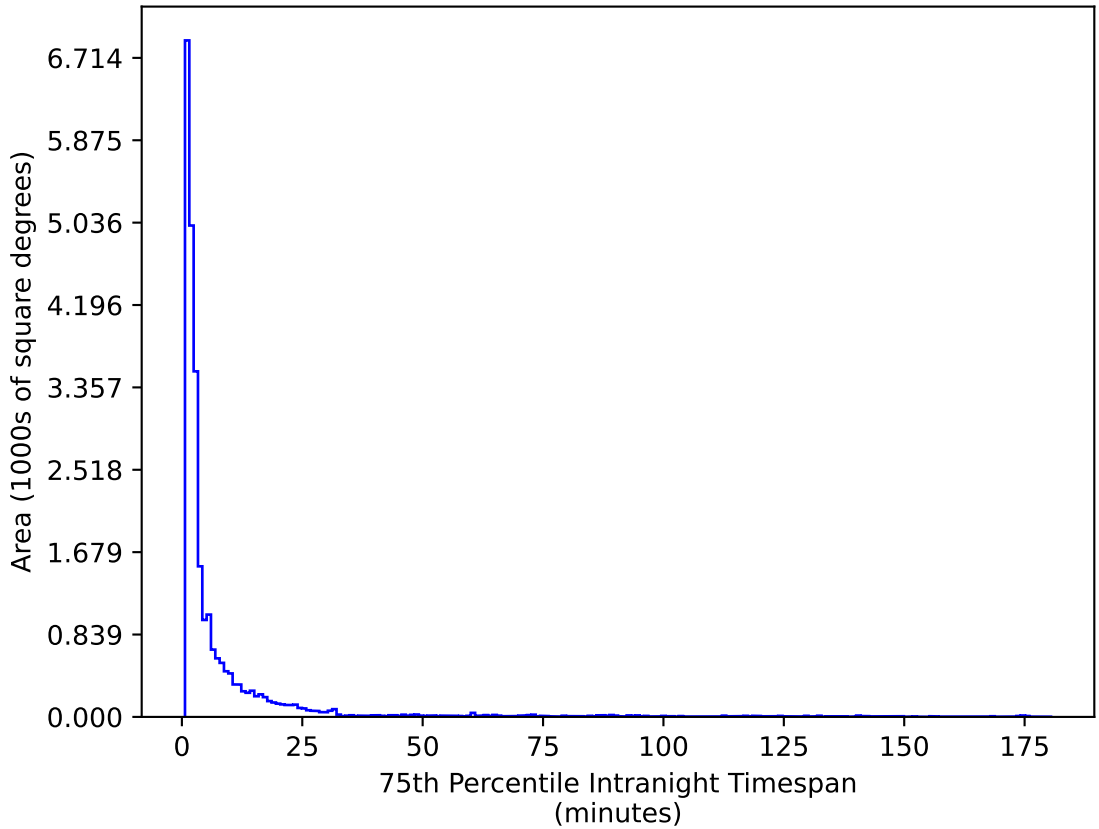
too_elab_r8_d3_gz_v3.4_10yrs All sky g band: 75th Percentile Intranight Timespan
