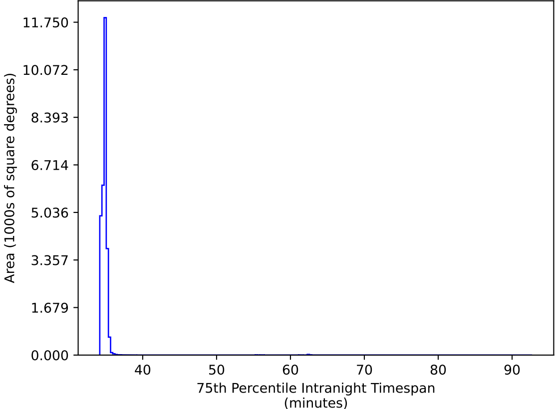
too_elab_r8_d3_gz_v3.4_10yrs All sky all bands: 75th Percentile Intranight Timespan
