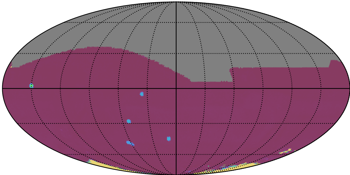
too_elab_r8_d3_gz_v3.4_10yrs All sky: 75th Percentile Intranight Timespan
