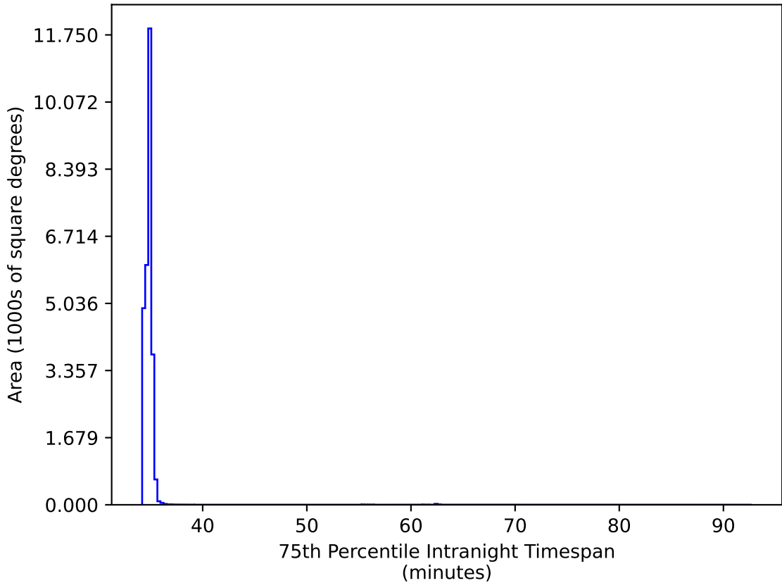
too_elab_r8_d3_gz_v3.4_10yrs All sky: 75th Percentile Intranight Timespan
