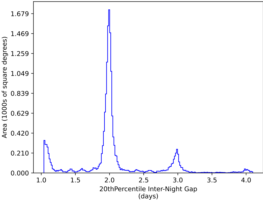
too_elab_r8_d3_gz_v3.4_10yrs WFD y band: 20thPercentile Inter-Night Gap
