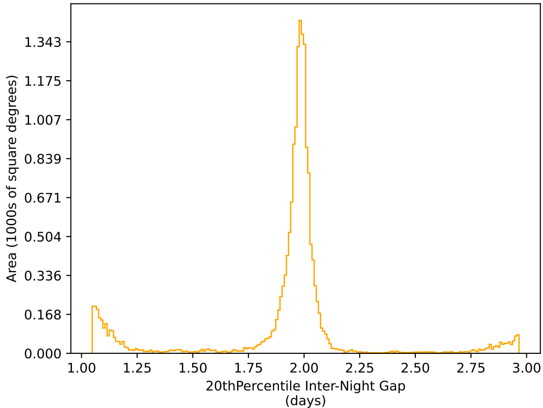
too_elab_r8_d3_gz_v3.4_10yrs WFD r band: 20thPercentile Inter-Night Gap
