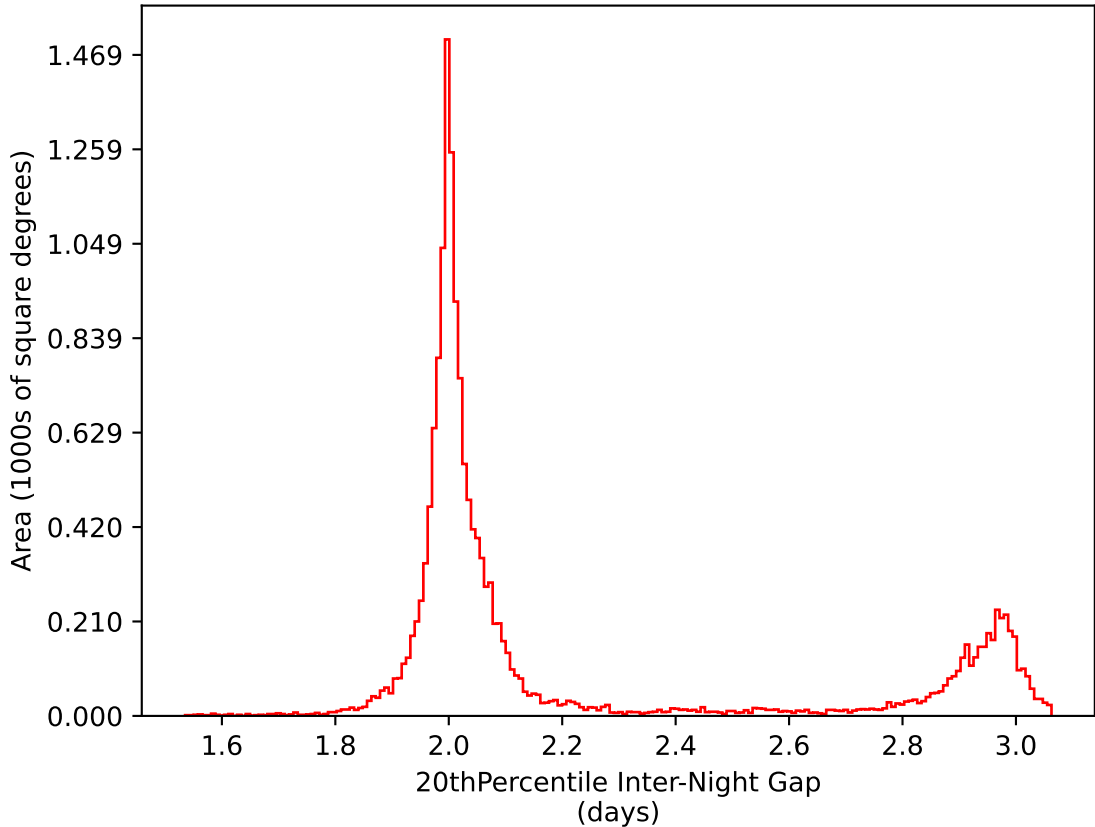
too_elab_r8_d3_gz_v3.4_10yrs WFD i band: 20thPercentile Inter-Night Gap
