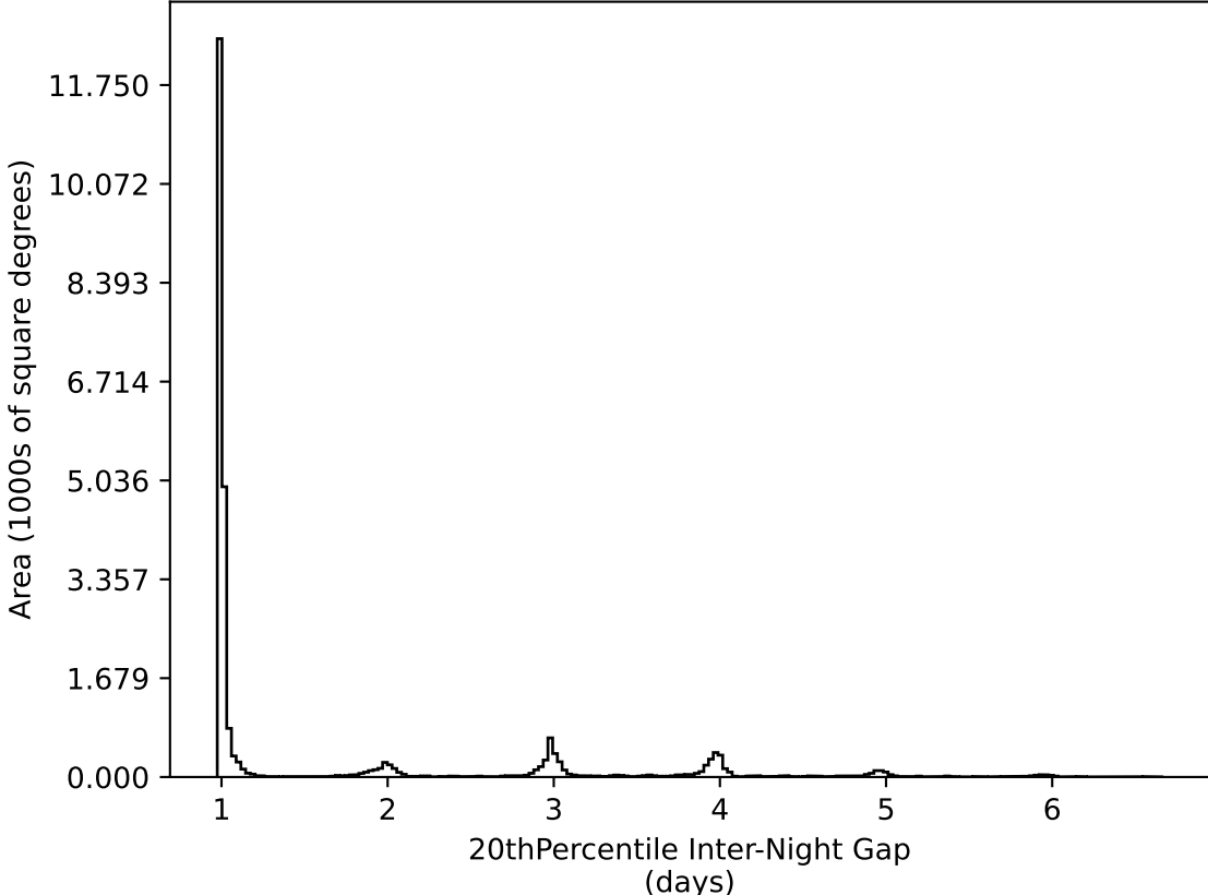
too_elab_r8_d3_gz_v3.4_10yrs All sky all bands: 20thPercentile Inter-Night Gap
