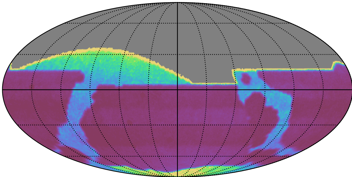
too_elab_r8_d3_gz_v3.4_10yrs : properMotion
