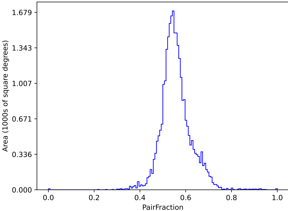
too_elab_r8_d3_gz_v3.4_10yrs (g or r or i): PairFraction
