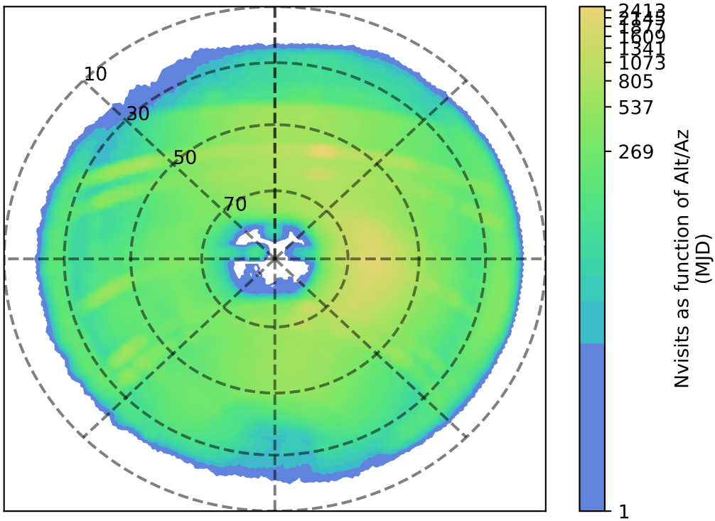
too_elab_r8_d3_gz_v3.4_10yrs z: Nvisits as function of Alt/Az
