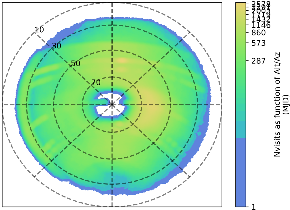
too_elab_r8_d3_gz_v3.4_10yrs r: Nvisits as function of Alt/Az
