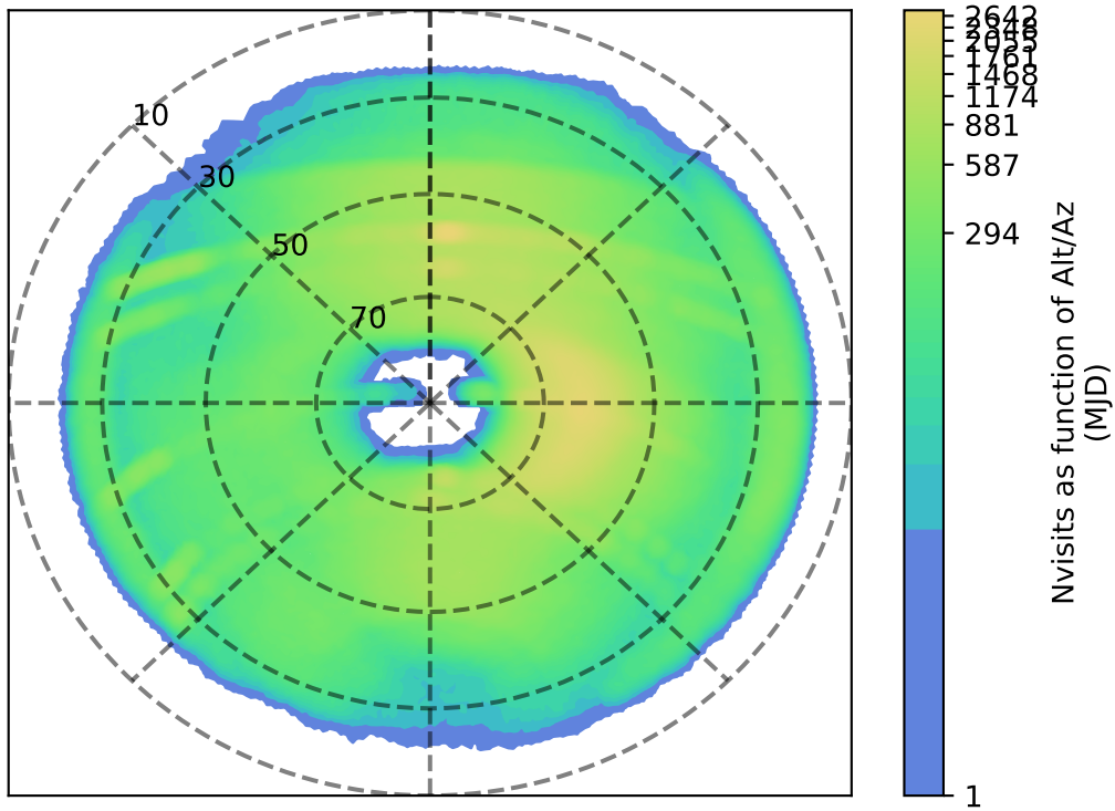
too_elab_r8_d3_gz_v3.4_10yrs i: Nvisits as function of Alt/Az
