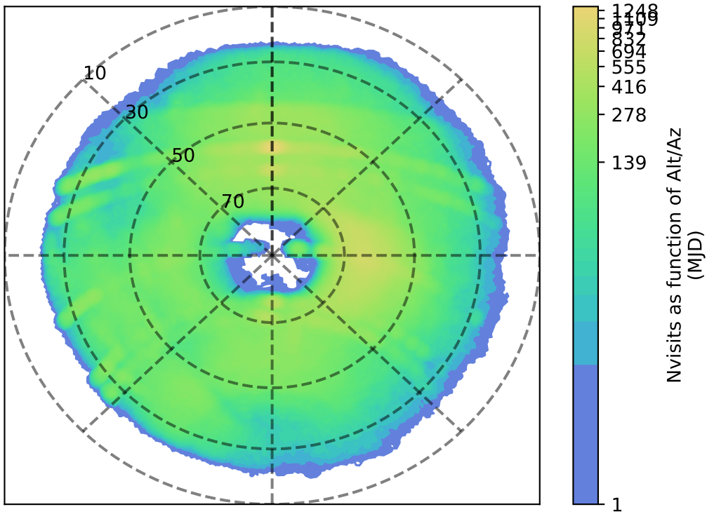
too_elab_r8_d3_gz_v3.4_10yrs g: Nvisits as function of Alt/Az
