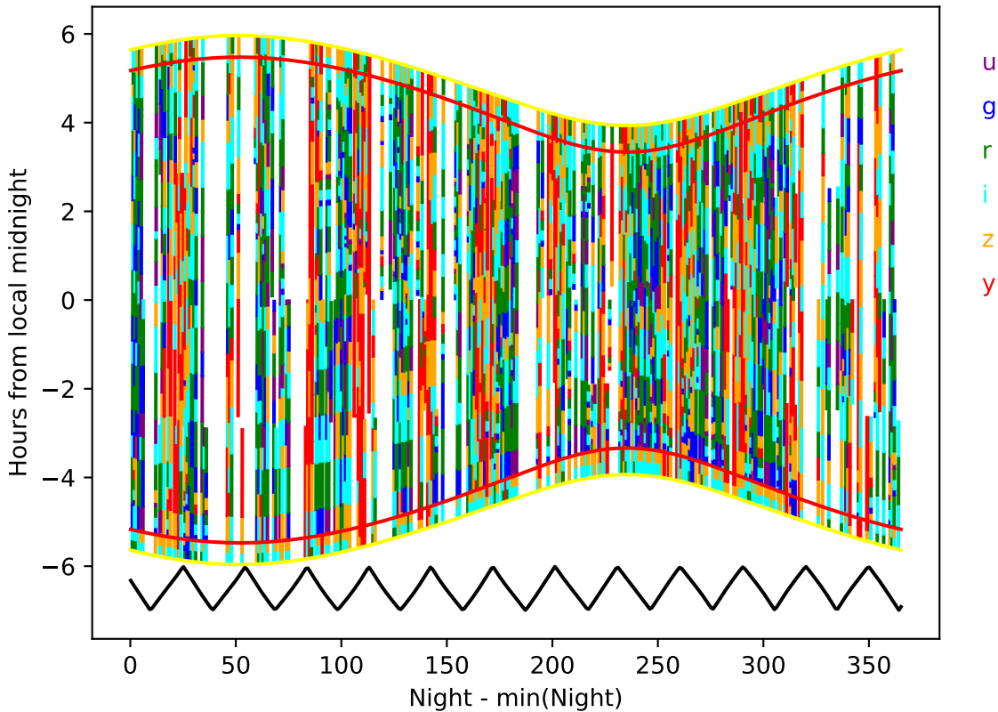
too_elab_r8_d3_gz_v3.4_10yrs year 7-8: Hourglass
