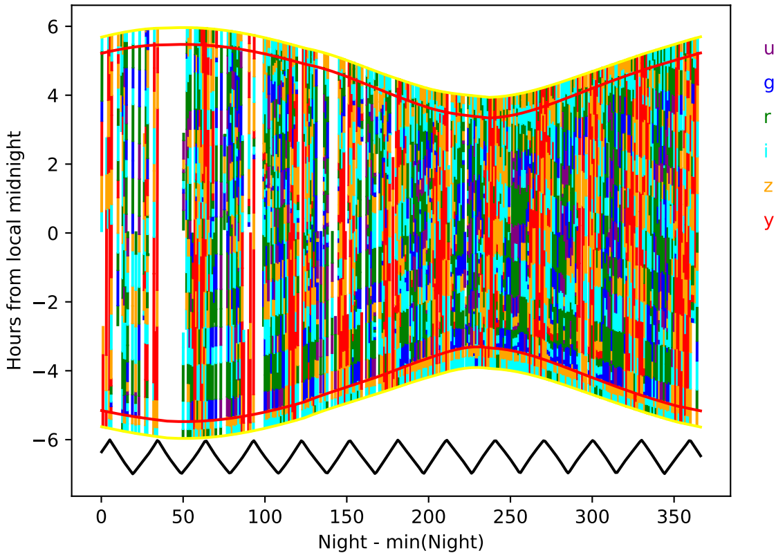
too_elab_r8_d3_gz_v3.4_10yrs year 6-7: Hourglass
