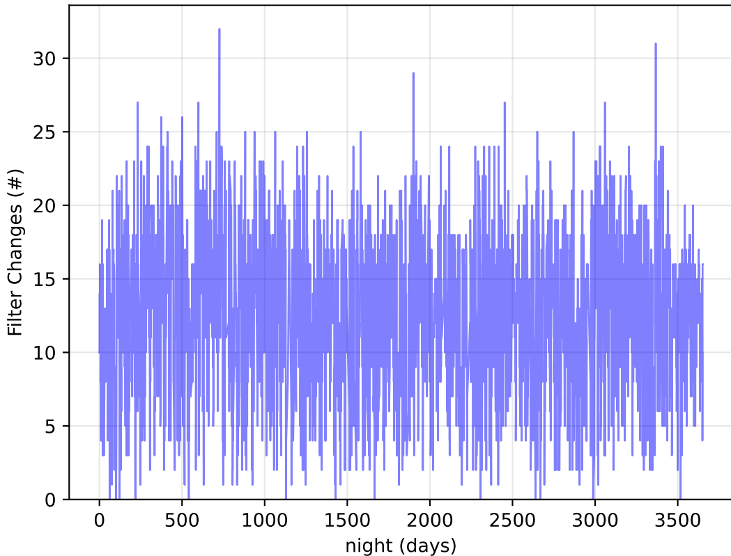
too_elab_r8_d3_gz_v3.4_10yrs : Filter Changes
