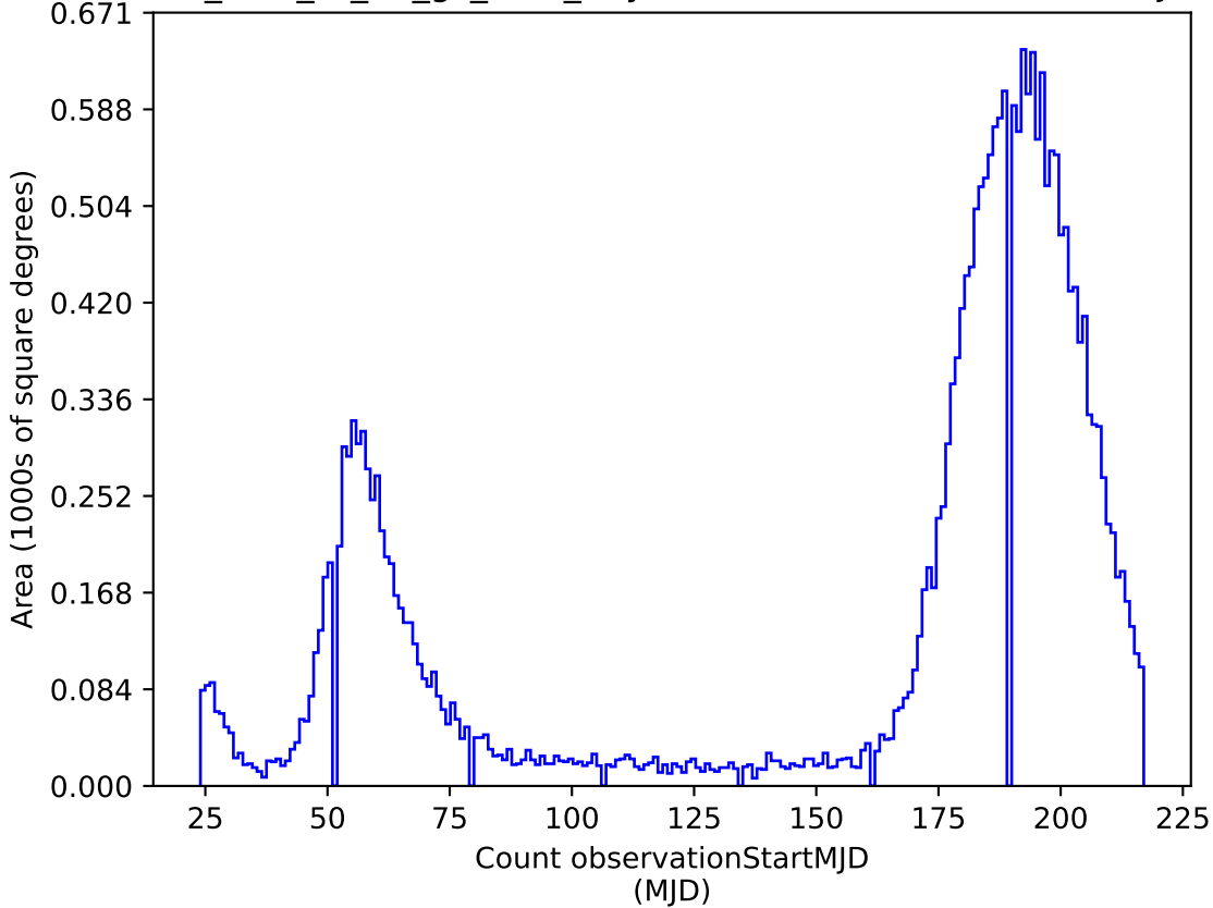
too_elab_r8_d3_gz_v3.4_10yrs i: Count observationStartMJD
